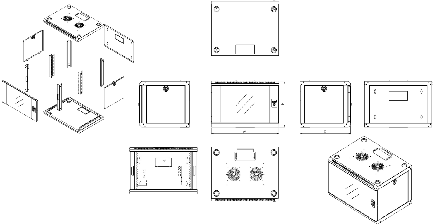
19" Atlas BASIC Wall Mount Cabinets W=600 D=450/600
